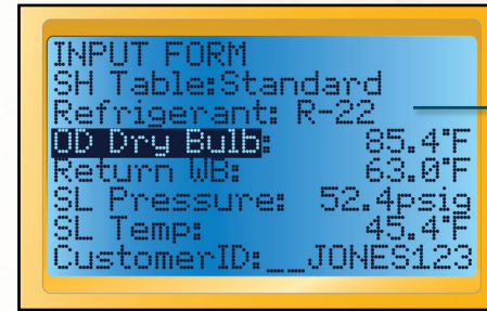
Superheat INPUT FORM using the Standard superheat table from Title 24.
