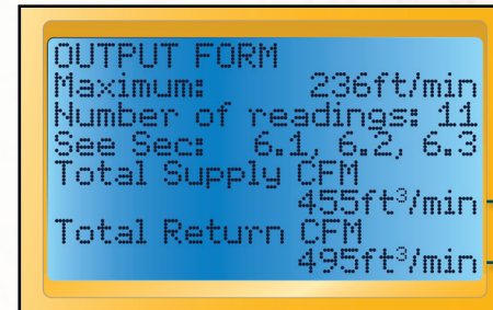
CFM OUTPUT FORM continued from above.
