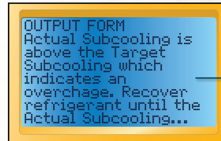
Subcooling OUTPUT FORM continued from above.
