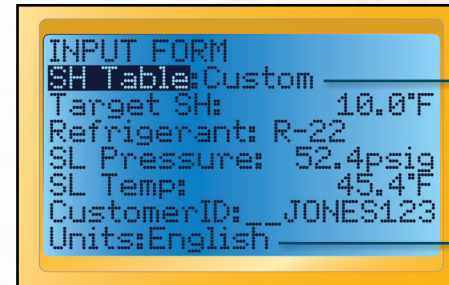
Superheat INPUT FORM using the Custom superheat table which allows the technician to enter in the manufacturer's recommended superheat.
