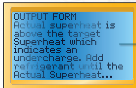
Superheat OUTPUT FORM continued from above.
