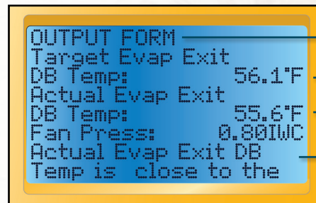
Target Evap Exit Temp OUTPUT FORM.
