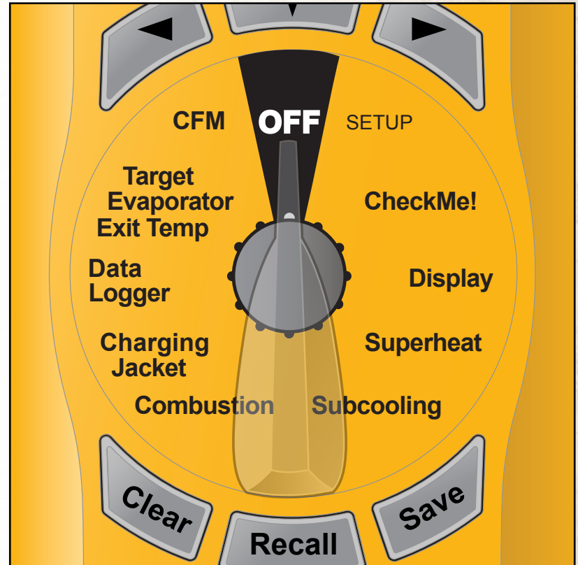
Select a test with the HG3 Dial.
