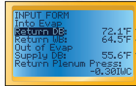
Target Evaporator Exit Temperature Test INPUT FORM filled.
