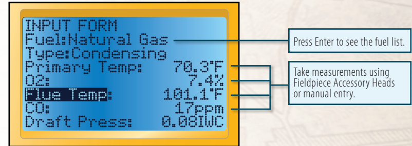
Combustion Analysis INPUT FORM.
