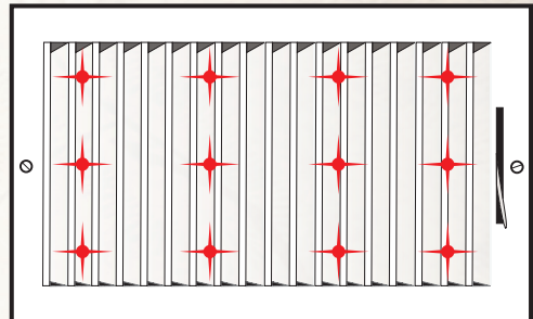
Traverse example for a rectangular grille.
